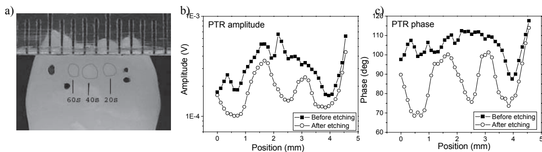
Figure 1. Photographs and experimental results of sample tooth T4. (a) Sample T4 showing 3 etched areas of 60 s, 40 s, and 20s respectively. (b) and (c) PTR amplitude and phase signals across the scanned line at 30Hz.
